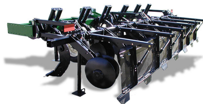
RIPPER BEDDER TILLAGE TOOL
